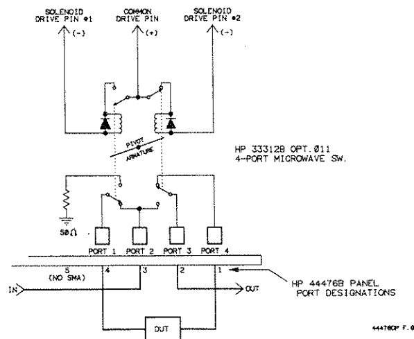
Figure 9. Transfer Switch Application.
